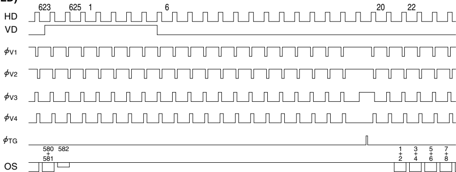
VERTICAL TRANSFER TIMING <NORMAL OUTPUT>
